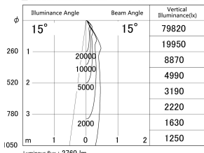
■ Direct Horizontal Illuminance DD139-3015MW9030D
