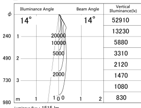
■ Direct Horizontal Illuminance DD139-1515MW9035D
