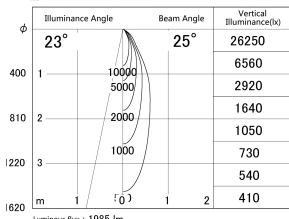
■ Direct Horizontal Illuminance DD139-2020MW9035D
