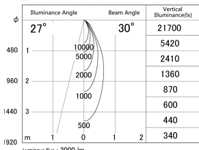
■ Direct Horizontal Illuminance DD139-2030MW9035D
