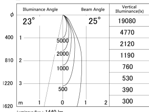
■ Direct Horizontal Illuminance DD139-1520MW9040D
