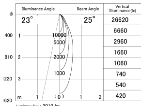
■ Direct Horizontal Illuminance DD139-2020MW9040D
