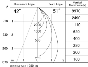
■ Direct Horizontal Illuminance DD139-2050MW9040D
