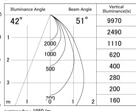
■ Direct Horizontal Illuminance DD139-2050MW9040D
