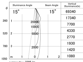
■ Direct Horizontal Illuminance DD139-2515MW9040D
