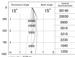
■ Direct Horizontal Illuminance DD139-3015MW9040D
