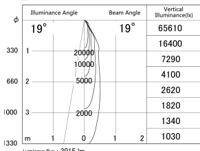
■ Direct Horizontal Illuminance DD139-3020MW9040D
