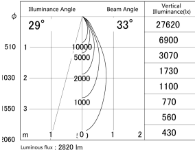
■ Direct Horizontal Illuminance DD139-3030MW9040D
