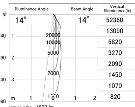
■ Direct Horizontal Illuminance DD139-1515MB9027D
