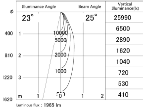
■ Direct Horizontal Illuminance DD139-2020MB9027D
