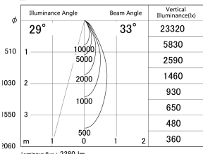
■ Direct Horizontal Illuminance DD139-2530MB9027D
