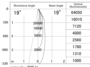
■ Direct Horizontal Illuminance DD139-3020MB9027D
