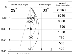
■ Direct Horizontal Illuminance DD139-3030MB9027D
