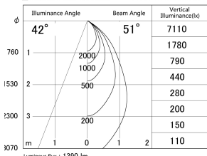
■ Direct Horizontal Illuminance DD139-1550MB9030D
