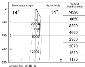
■ Direct Horizontal Illuminance DD139-2015MB9030D
