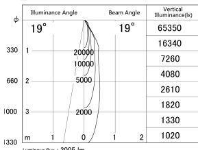
■ Direct Horizontal Illuminance DD139-3020MB9030D
