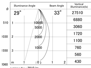
■ Direct Horizontal Illuminance DD139-3030MB9030D
