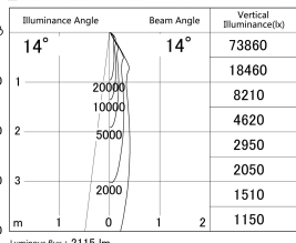
■ Direct Horizontal Illuminance DD139-2015MB9035D
