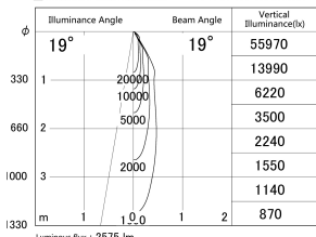
■ Direct Horizontal Illuminance DD139-2520MB9035D
