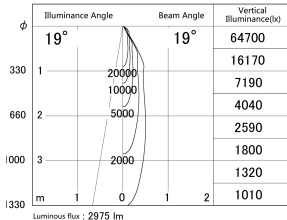
■ Direct Horizontal Illuminance DD139-3020MB9035D
