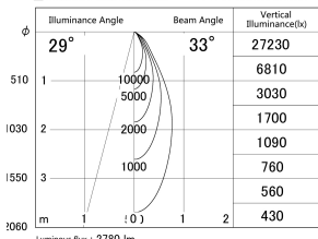
■ Direct Horizontal Illuminance DD139-3030MB9035D
