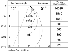
■ Direct Horizontal Illuminance DD139-3050MB9035D
