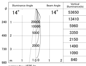
■ Direct Horizontal Illuminance DD139-1515MB9040D
