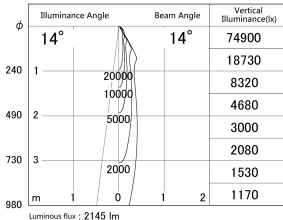
■ Direct Horizontal Illuminance DD139-2015MB9040D
