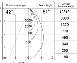
■ Direct Horizontal Illuminance DD139-2550MB9040D
