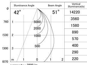
■ Direct Horizontal Illuminance DD139-3050MB9040D
