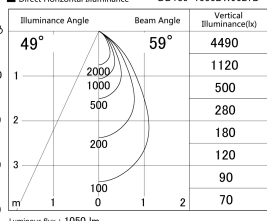
■ Direct Horizontal Illuminance DD139-1550DW9027D
