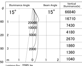
■ Direct Horizontal Illuminance DD139-3015DW9027D
