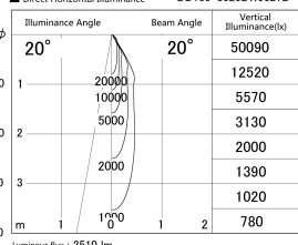
■ Direct Horizontal Illuminance DD139-3020DW9027D
