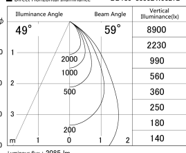
■ Direct Horizontal Illuminance DD139-3050DW9027D
