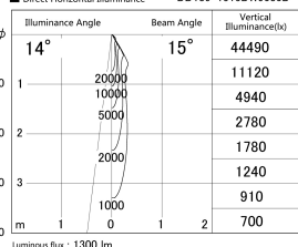
■ Direct Horizontal Illuminance DD139-1515DW9030D
