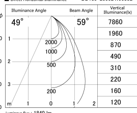
■ Direct Horizontal Illuminance DD139-2550DW9030D
