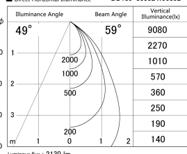
■ Direct Horizontal Illuminance DD139-3050DW9030D
