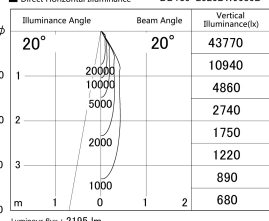
■ Direct Horizontal Illuminance DD139-2520DW9035D
