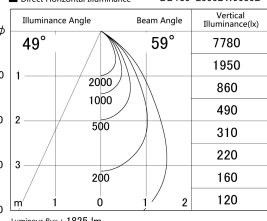
■ Direct Horizontal Illuminance DD139-2550DW9035D
