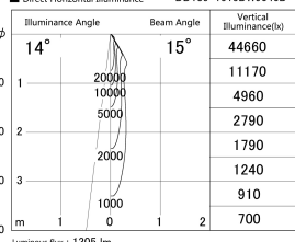
■ Direct Horizontal Illuminance DD139-1515DW9040D
