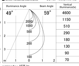
■ Direct Horizontal Illuminance DD139-1550DW9040D
