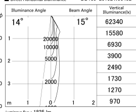
■ Direct Horizontal Illuminance DD139-2015DW9040D
