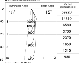
■ Direct Horizontal Illuminance DD139-2515DW9040D
