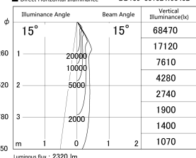
■ Direct Horizontal Illuminance DD139-3015DW9040D
