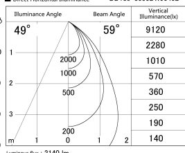
■ Direct Horizontal Illuminance DD139-3050DW9040D
