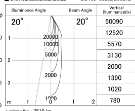
■ Direct Horizontal Illuminance DD139-3020DB9027D
