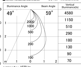
■ Direct Horizontal Illuminance DD139-1550DB9030D
