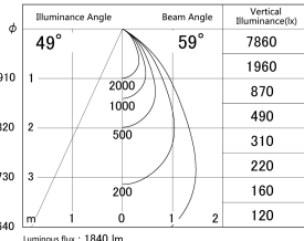
■ Direct Horizontal Illuminance DD139-2550DB9030D
