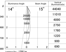
■ Direct Horizontal Illuminance DD139-1515DB9035D
