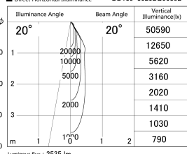
■ Direct Horizontal Illuminance DD139-3020DB9035D
