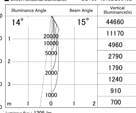
■ Direct Horizontal Illuminance DD139-1515DB9040D
